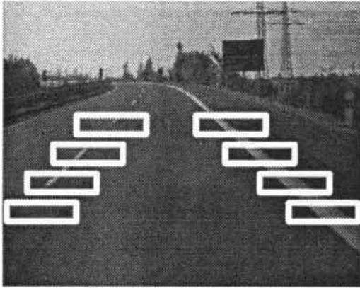
Fig. 5: Window positions for street edge tracking during automated navigation on public streets test vehicle at a speed close to 100km/h on a freeway and up to 60 km/h on an unmarked two-lane country road.
