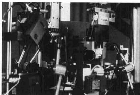
Fig. 1: Arrangement of cameras and illumination in a soldered joint inspection system (Viscom)
