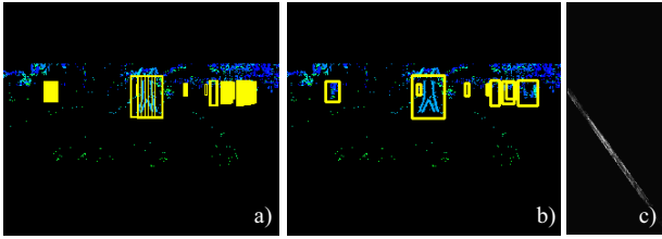
Figure 6. Results of the middle resolution step: a) “Obstacle pixels” disparity map with represented small ROIs, b) same image with merged ROIs, c) “road pixels” v -disparity image.
